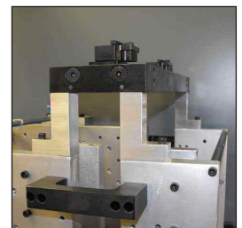
Channel Extenders
